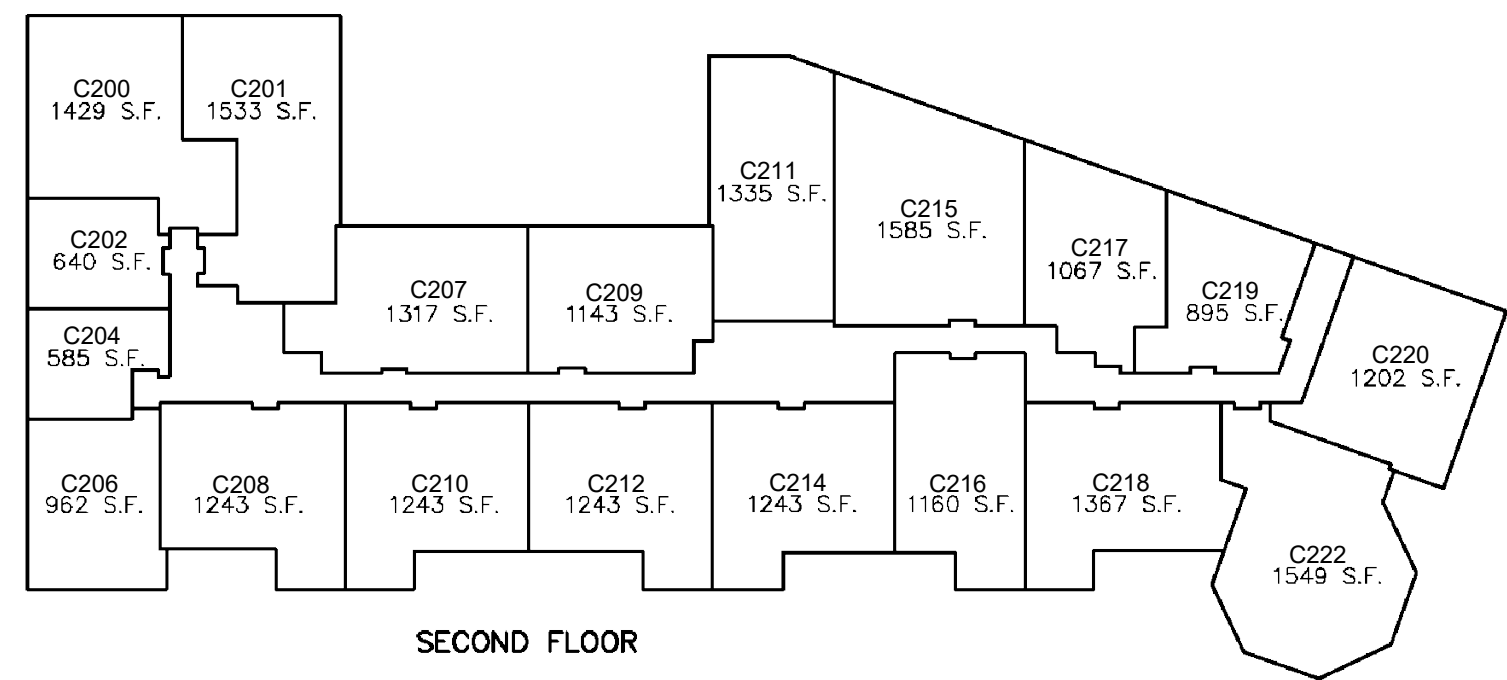
SECOND FLOOR
